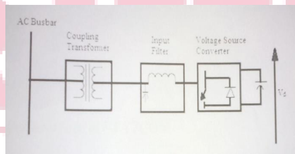
Figure.1 Circuit with STATCOM
