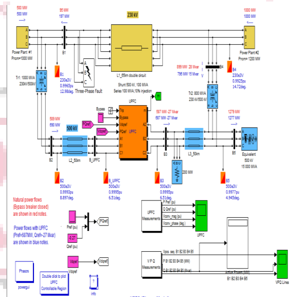
Figure.4 Power entity Model with UPFC
