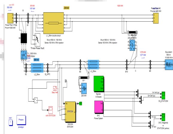
Figure.5 Power entity Model for STATCOM
