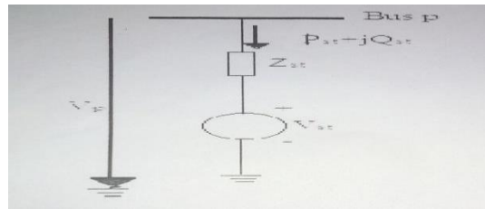
Figure.3 Equivalent circuit of a STATCOM
