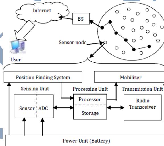
Figure 1: System Model of Wireless Sensor Network [4]
