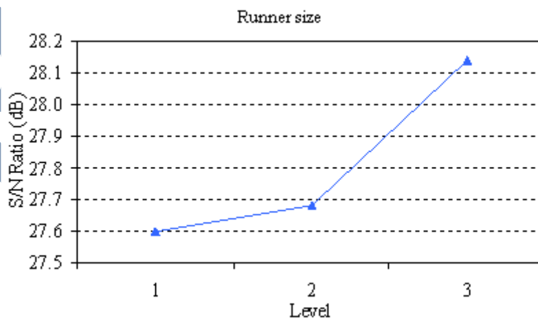
Figure 2c. Main effects plot for runner size S/N ratio values on impact energy
