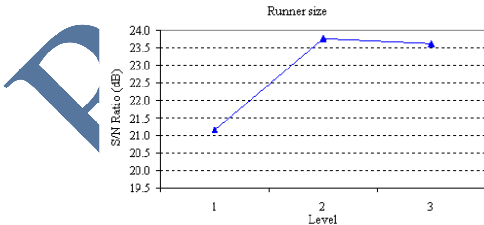
Figure 1c. Main effects plot for runner size S/N ratio values on hardness
