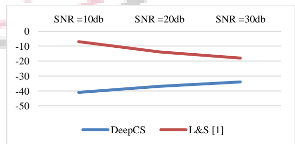
Figure 4: MSE Comparative Analysis with Existing Work
